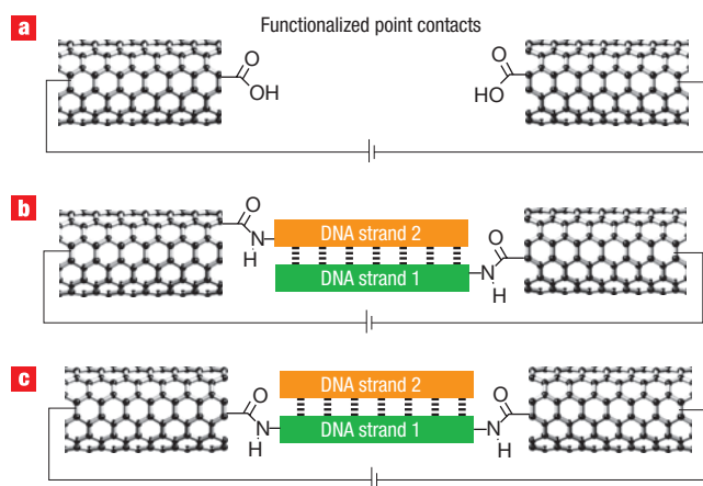
Figure 1 A method to cut and functionalize individual SWNTs with DNA strands. a , Functionalized point contacts made through the oxidative cutting of a SWNT wired into a device. b , Bridging by functionalization of both strands with amine functionality. c , Bridging by functionalization of one strand with amines on either end.
