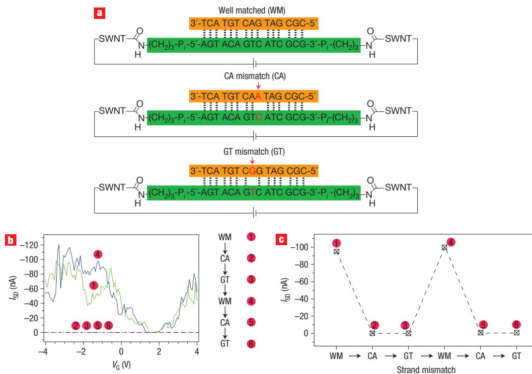
Figure 3 Mismatches have a large effect on DNA conductance. a , Replacing well-matched (WM) duplexes with CA and GT mismatches. b , Source–drain current versus V_G at a constant source–drain voltage (50 mV) for a SWNT device taken through the sequence 1 through 6. The current levels for points 2, 3, 5 and 6 are \sim 300 times lower. c , Source–drain current at V_G = -3 V at a constant source–drain voltage (50 mV) for the sequence 1 through 6.
