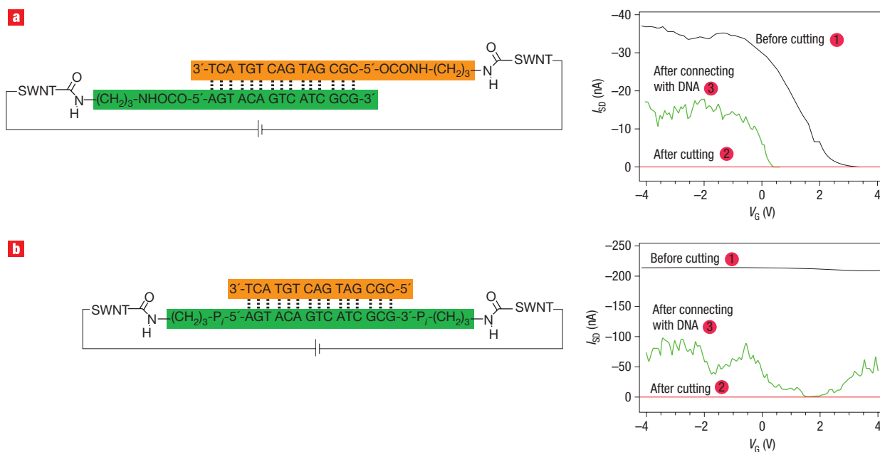
Figure 2 Device characteristics for individual SWNTs connected with DNA. a, b , Source–drain current versus V_G at a constant source–drain voltage (50 mV) before cutting (black curve: 1), after cutting (red curve: 2) and after connection with the DNA sequence shown (green curve: 3), for a semiconducting SWNT device ( a ) and a metallic SWNT device ( b ). Guanine, G; cytosine, C; adenine, A; thymine, T.
