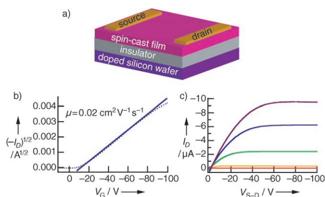
Figure 1. a) Schematic diagram of a field-effect transistor that was fabricated by evaporating source and drain electrodes onto a spin-cast film of 1c . b) Transconductance: the blue line is a fit of the linear portion of the data points (the source–drain voltage V_{S-D} was held at -60 V). c) Transistor output for thin-film transistors from 1c .
