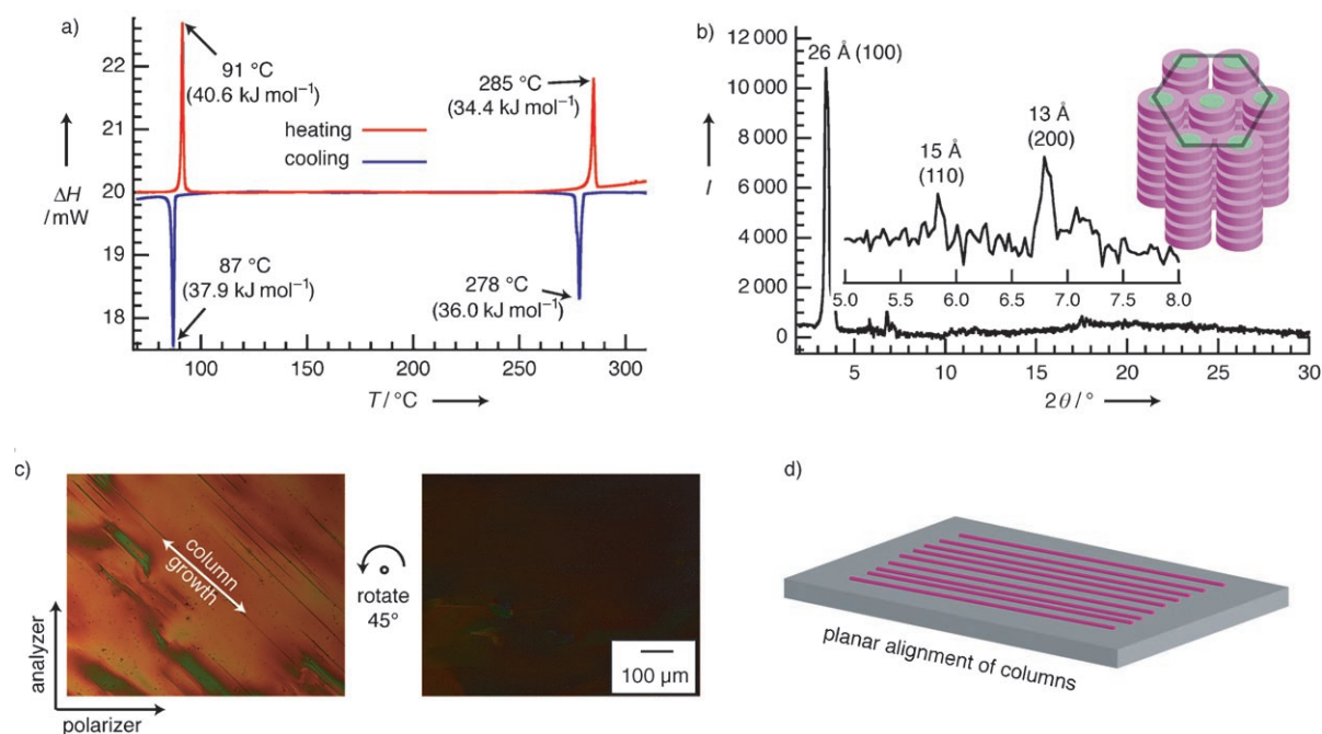
Figure 2. a) DSC trace of 1c (scan rate = 5^{\circ}\text{C min}^{-1} ) showing a mesophase. b) X-ray diffraction studies of 1c cooled into its mesophase from 295 to 120^{\circ}\text{C} and a hexagonal lattice of columns. c) Polarized light micrograph of 1c cooled into its mesophase which shows a planar alignment of columns that are extinguished when aligned with the polarizer or analyzer axes. The cooling rate was 5^{\circ}\text{C min}^{-1} , and the exposure time was the same for each picture. d) Schematic diagram of columns aligned parallel to the surface.
