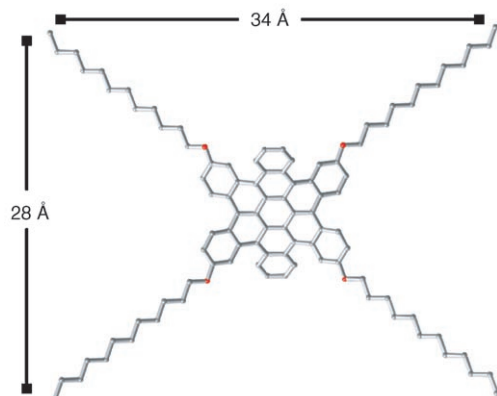
Figure 3. Molecular model of 1c with its side chains fully extended.
