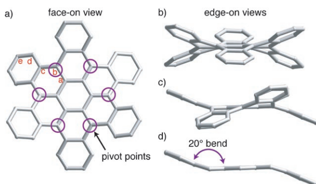
Figure 4. Crystal structure of 1a grown from 1,2,4-trichlorobenzene. Hydrogen atoms have been removed for clarity. a) Face-on view with marked pivot points (magenta circles). The C_a-C_b bond is relatively short and the C_b-C_c bond is relatively long. Side views are given in (b) and (c). d) Side view of one of the acene segments extracted from the crystal structure. The other atoms of the HBC are hidden from view.
